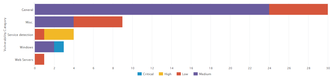
Graph: Vulnerability Category by Port
