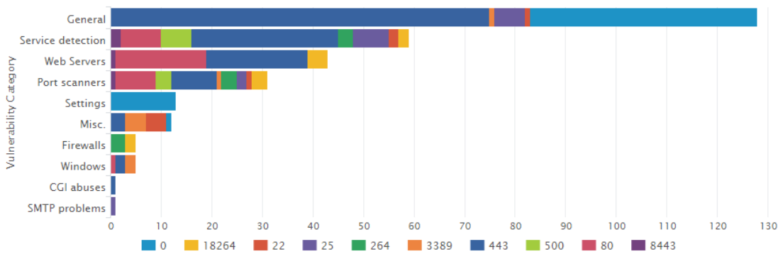
Graph: Vulnerability Category by Protocol
