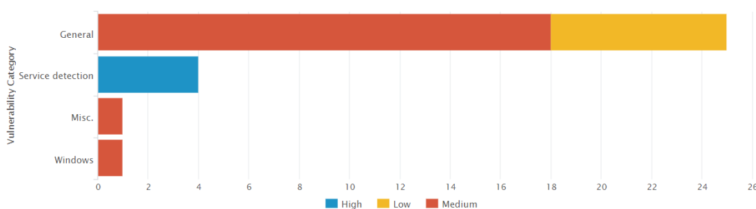
Graph: Vulnerability Category by Port
