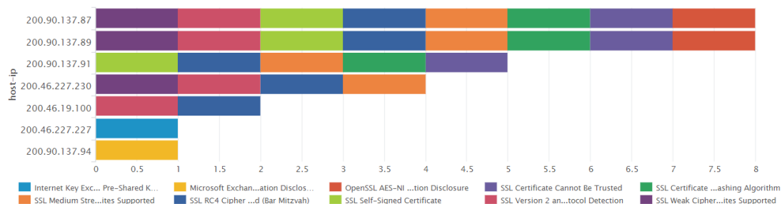
Graph: Host by Vulnerability Category
