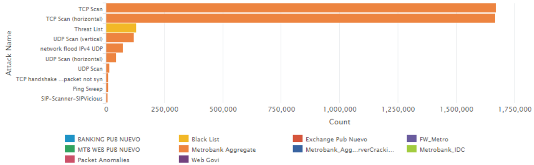
Graph: Top Attacks Blocked by Destination
