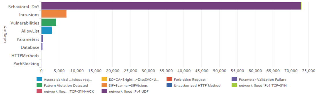
Graph: Top Attacked Destinations Blocked
