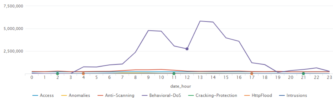
Graph: Top Attacks Blocked by Bandwidth
