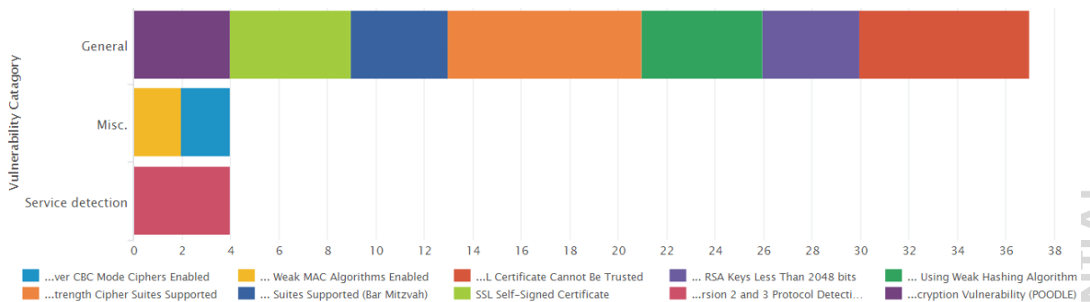
Graph: Vulnerability Category by Host
