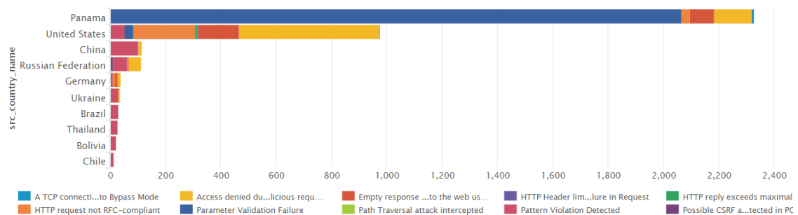
Graph: Attacks Types Blocked by Week - AppWall
